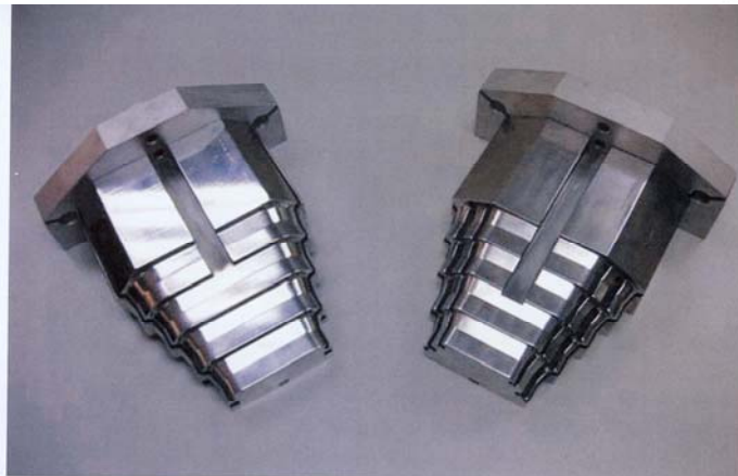
WINDING FORMS FOR STATOMAT MACHINE FW1/600
